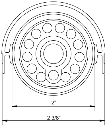
Front View (LED 12 pieces)
